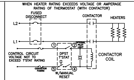
TYPICAL WIRING WITH 3 ELEMENTS USING A DOUBLE POLE THERMOSTAT
