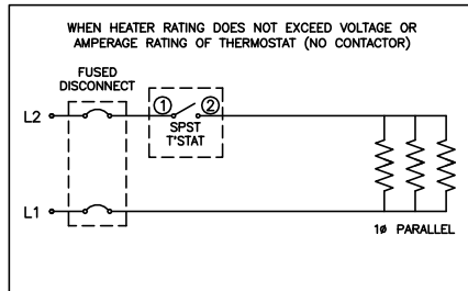
TYPICAL WIRING WITH 3 ELEMENTS USING A SPST THERMOSTAT
