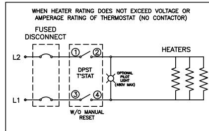
TYPICAL WIRING WITH 3 ELEMENTS USING A DOUBLE POLE THERMOSTAT
